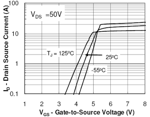
Transfer Characteristic
