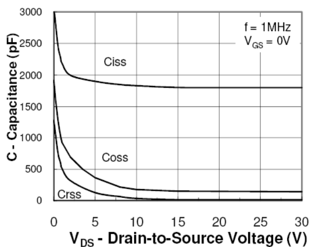
Capacitance
